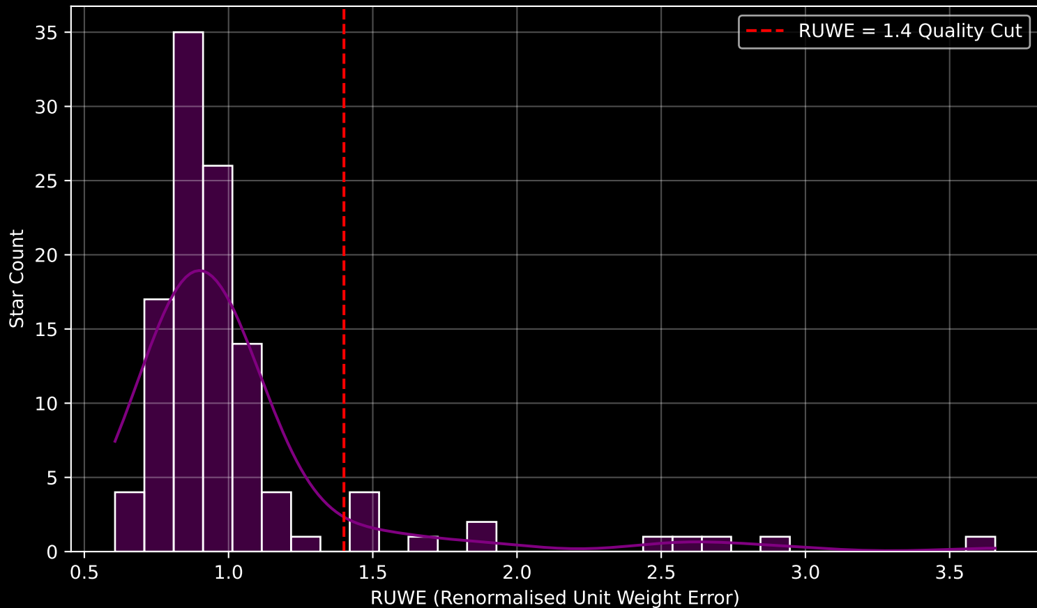
GAPOGEE DR17 Field [282-32-O_TESS] RUWE Distribution (n= 113)
