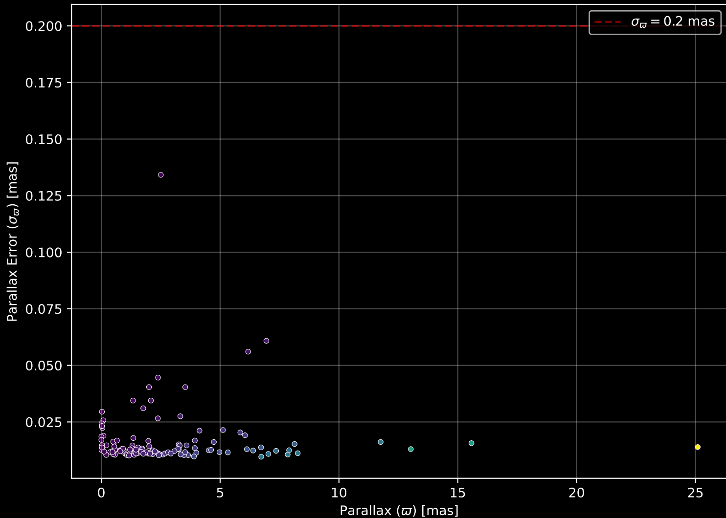
APOGEE DR17 Field: [282-32-O_TESS] Parallax Quality (n= 115)
