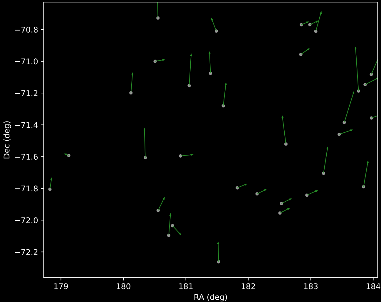
APOGEE DR17 Cluster 4 Proper Motion Vectors (n=33)
