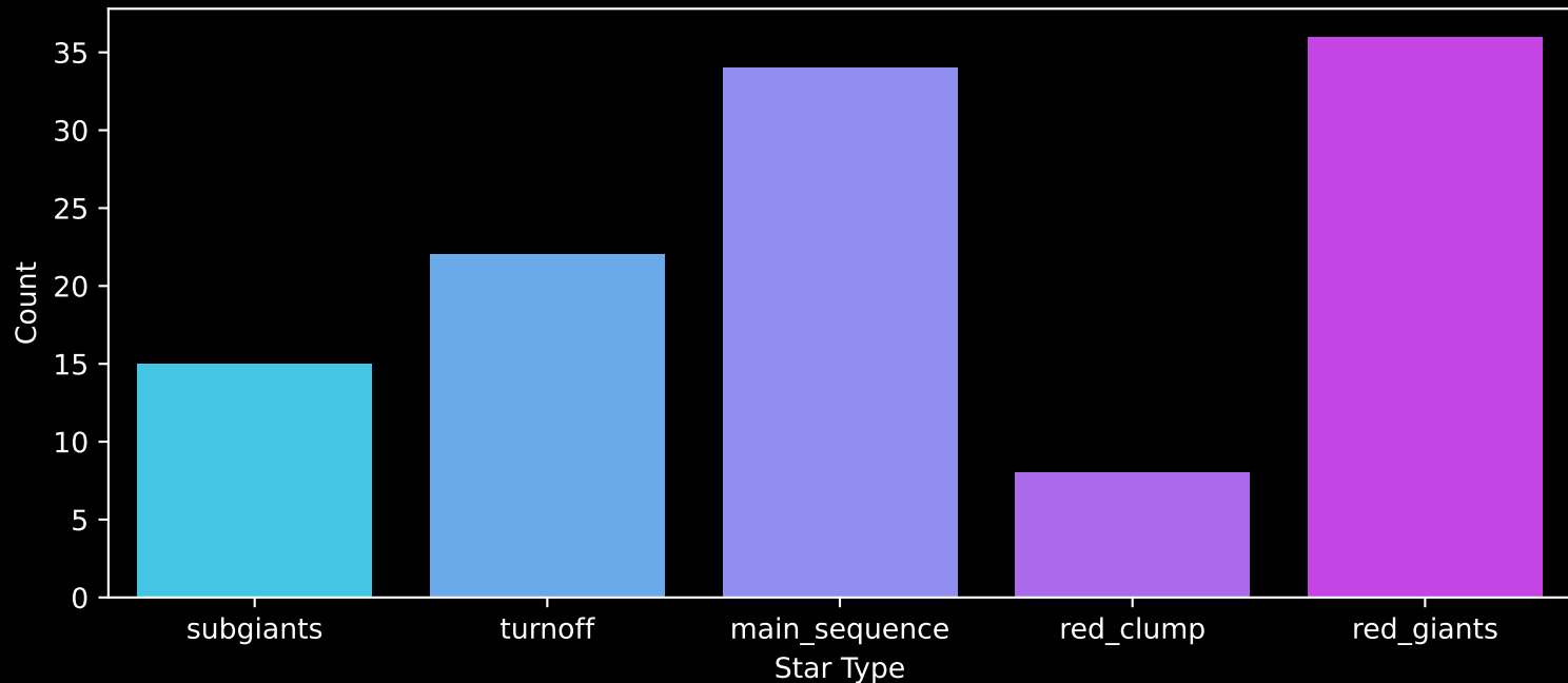
APOGEE DR17 Field: [282-32-O_TESS] Count plot of Star Type
